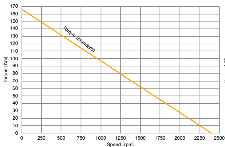
Torque curves
