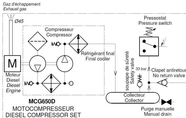
SCHEMA DE PRINCIPE PRINCIPLE DIAGRAM
