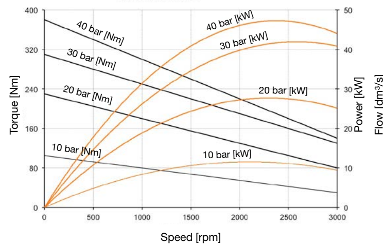
TORQUE / SPEED / POWER DIAGRAM
