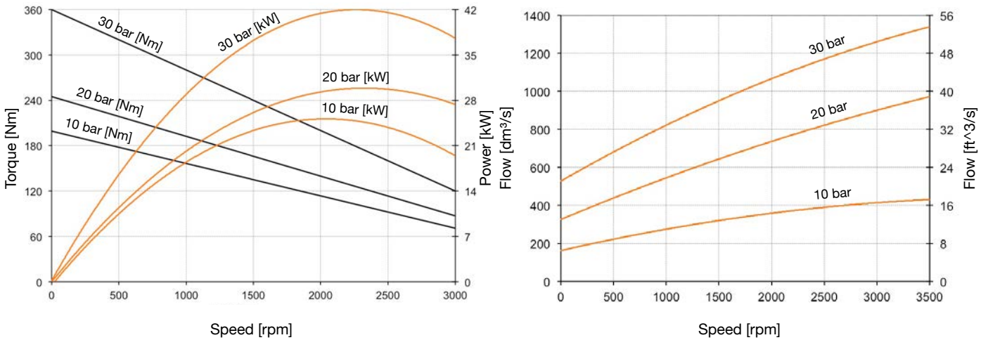
TORQUE / SPEED / POWER DIAGRAM
