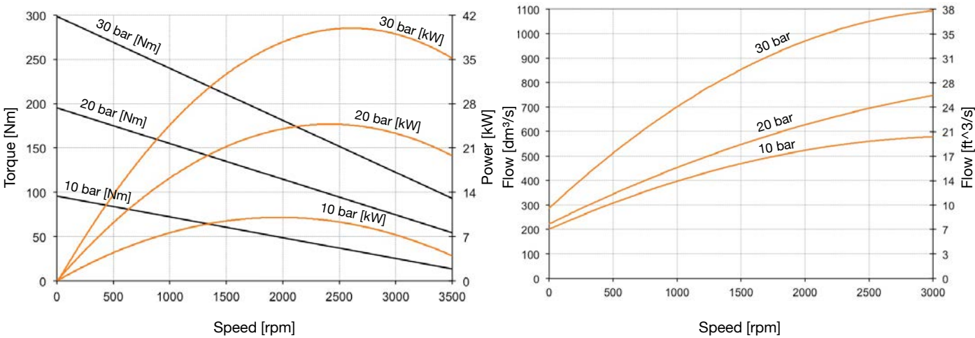
TORQUE / SPEED / POWER DIAGRAM
